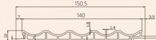
配套产品截面图 Products Sectional View Item: M1150内圆板
