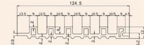
配套产品截面图 Products Sectional View Item: M12413格栅
