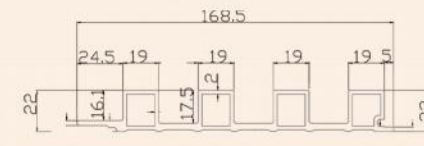
配套产品截面图 Products Sectional View Item: M170格栅
