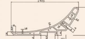
配套产品截面图 Products Sectional View Item: H150大怀抱
