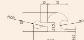
配套产品截面图 Products Sectional View Item:H52圆弧
