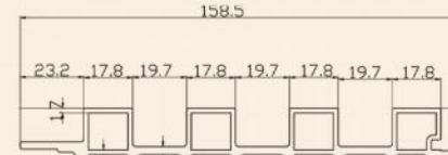
配套产品截面图 Products Sectional View Item: M150小格栅
