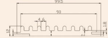
配套产品截面图 Products Sectional View Item:M100波浪板
