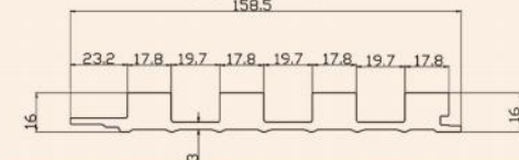
配套产品截面图 Products Sectional View Item: S1516 实心格栅
