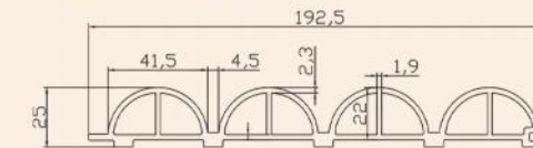
配套产品截面图 Products Sectional View Item: M192大四圆
