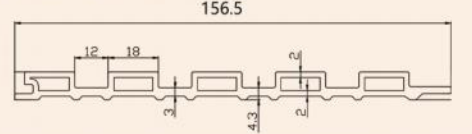
配套产品截面图 Products Sectional View Item: M159小长城
