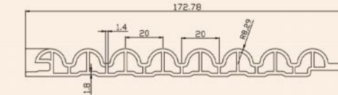
配套产品截面图 Products Sectional View Item: M172小圆板
